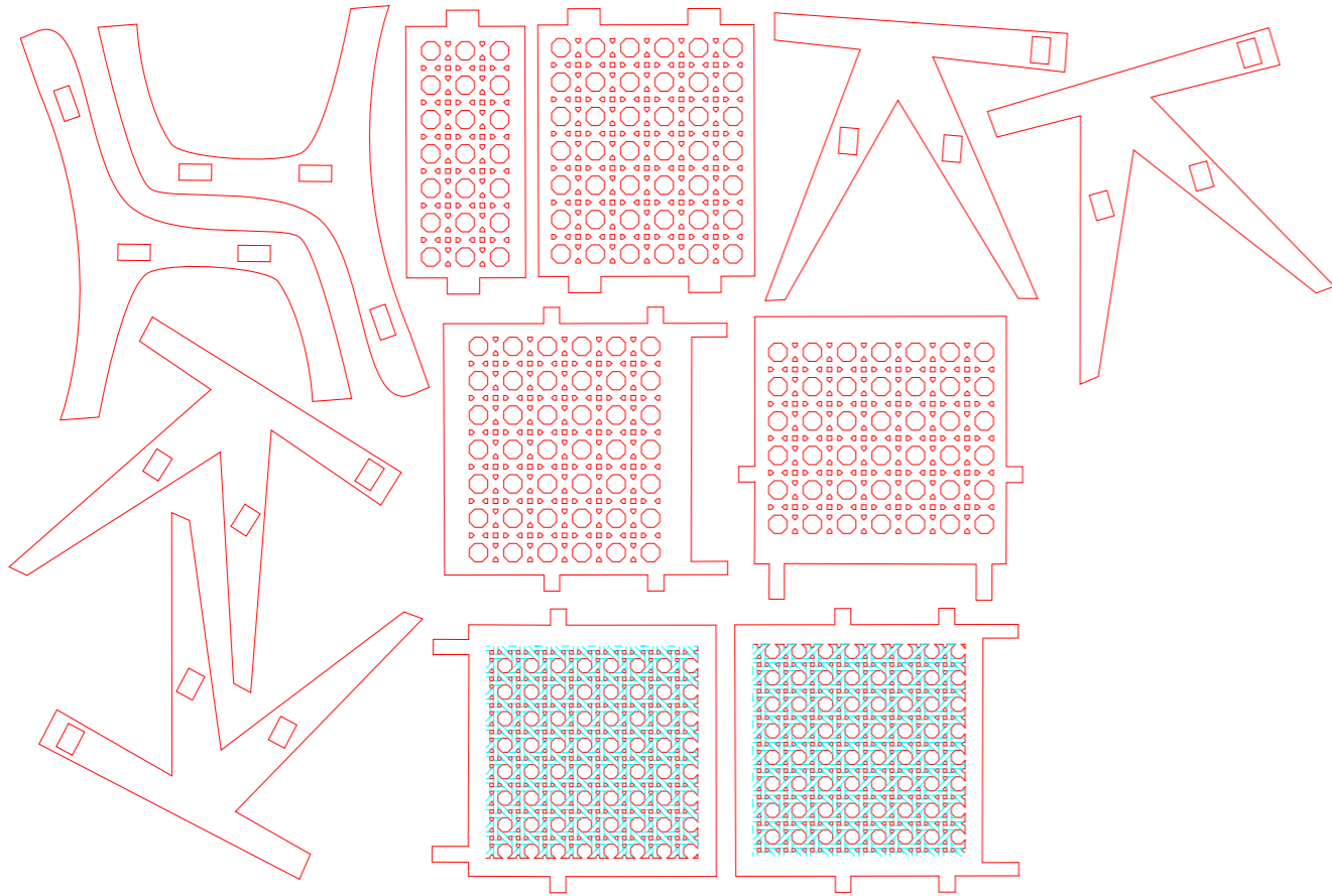
Rattan Chair Design
