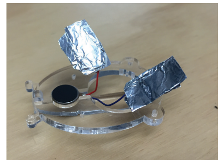
6. Fold aluminium foil around motor wires (for improved conductivity).
