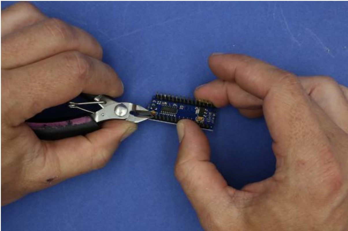
Half-way there - this is pins D10,D9,D8 and Ground
